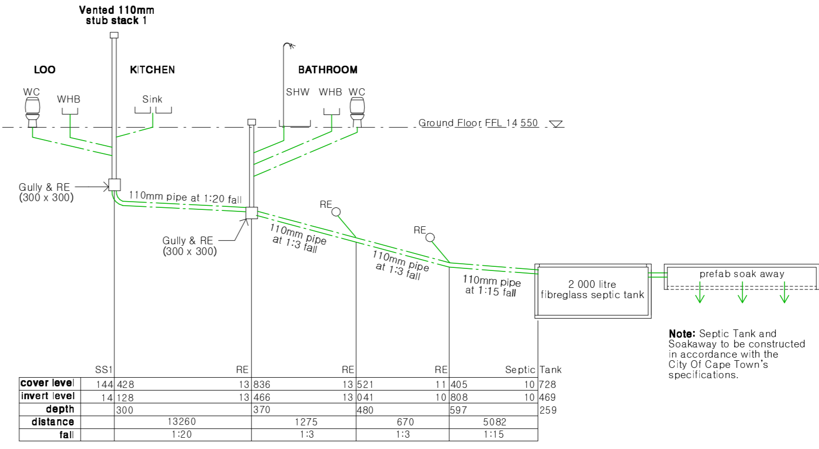
2 Drainage section Not to scale
